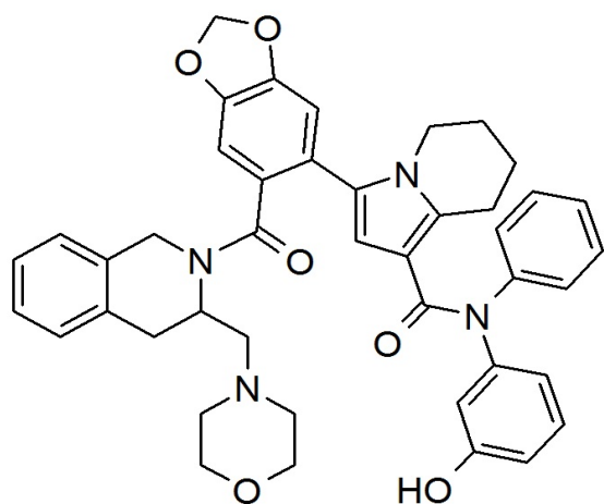
PC-6350201, Methanol-D4
